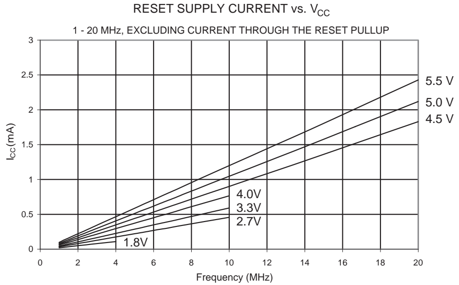
Figure 23-45. Reset Supply Current vs. V_{CC} (1 - 20 MHz, Excluding Current Through the Reset Pull-up)
