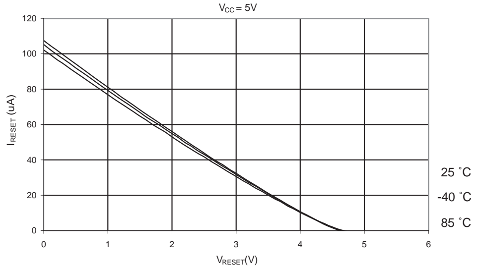
Figure 23-19. Reset Pull-up Resistor Current vs. Reset Pin Voltage ( V_{CC} = 5V )
